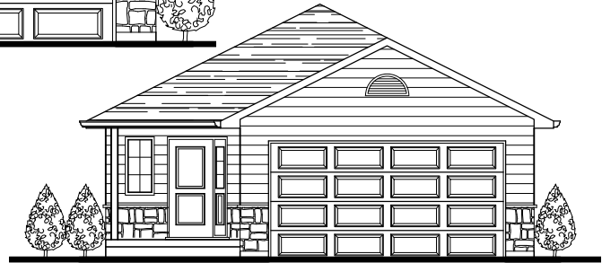
FRONT ELEVATION 'B'
