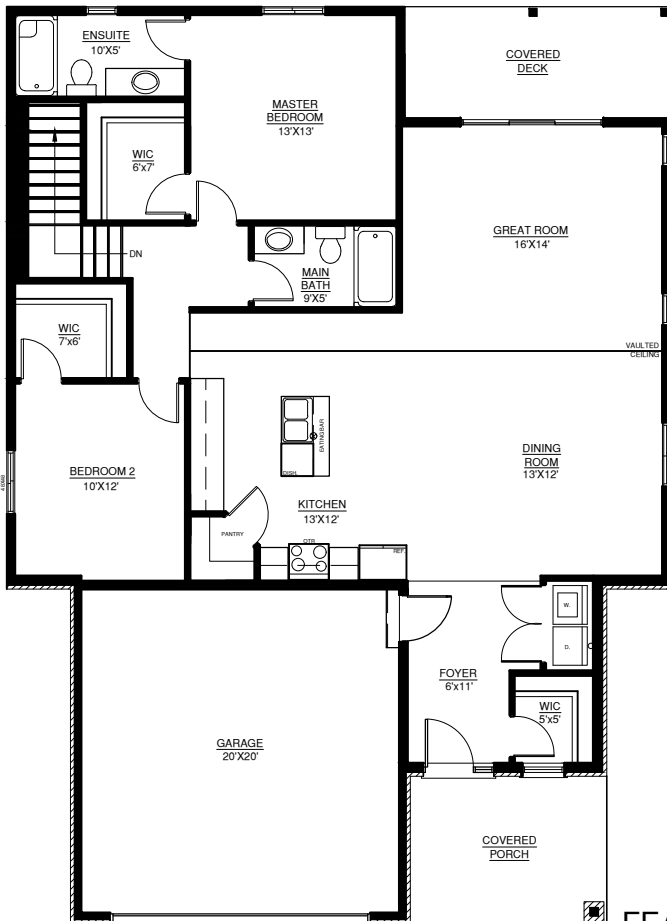
GROUND FLOOR PLAN 41'-8"X57'-6"
