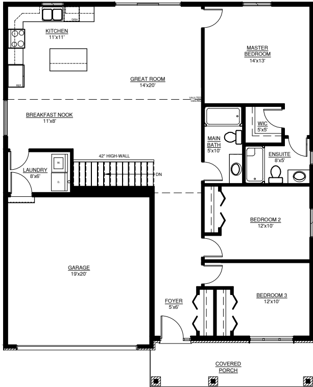
GROUND FLOOR PLAN 41'-10"X51'-10"
