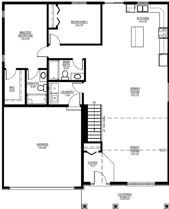
GROUND FLOOR PLAN 41'-10"X51'-10"
