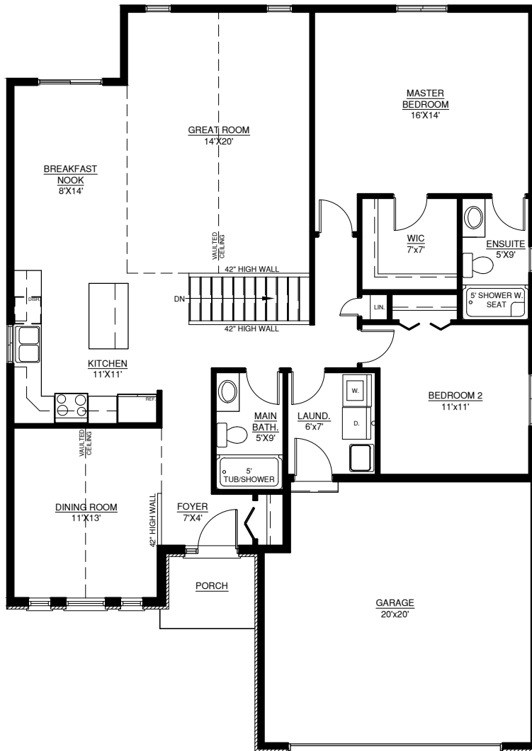
GROUND FLOOR PLAN 40'-4"X57'-0"
