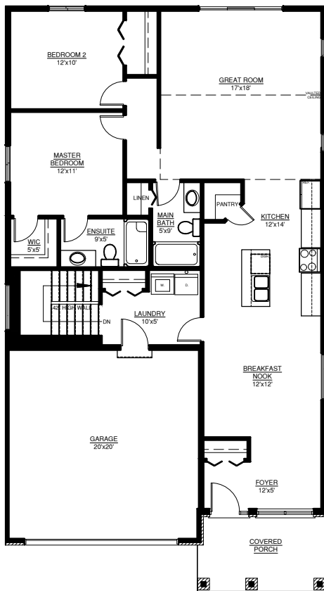
GROUND FLOOR PLAN 34'-0"X62'-0"
