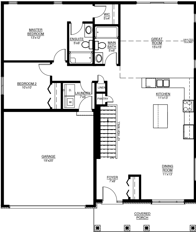
GROUND FLOOR PLAN 41'-8"X49'-2"
