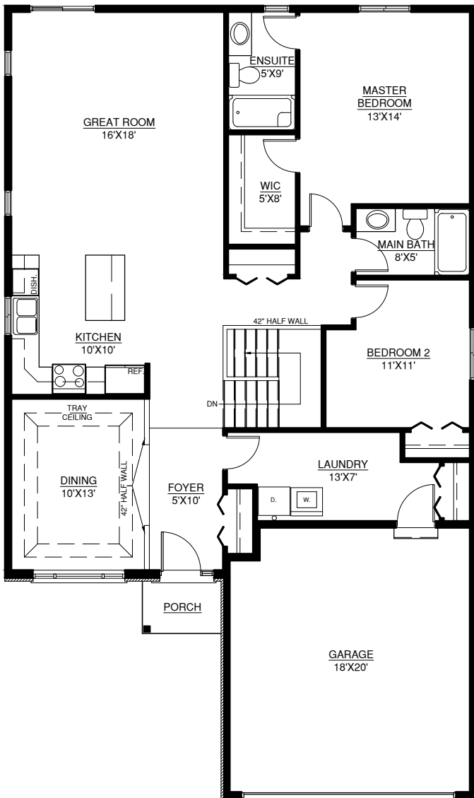
GROUND FLOOR PLAN 36'-10"X60'-0"
