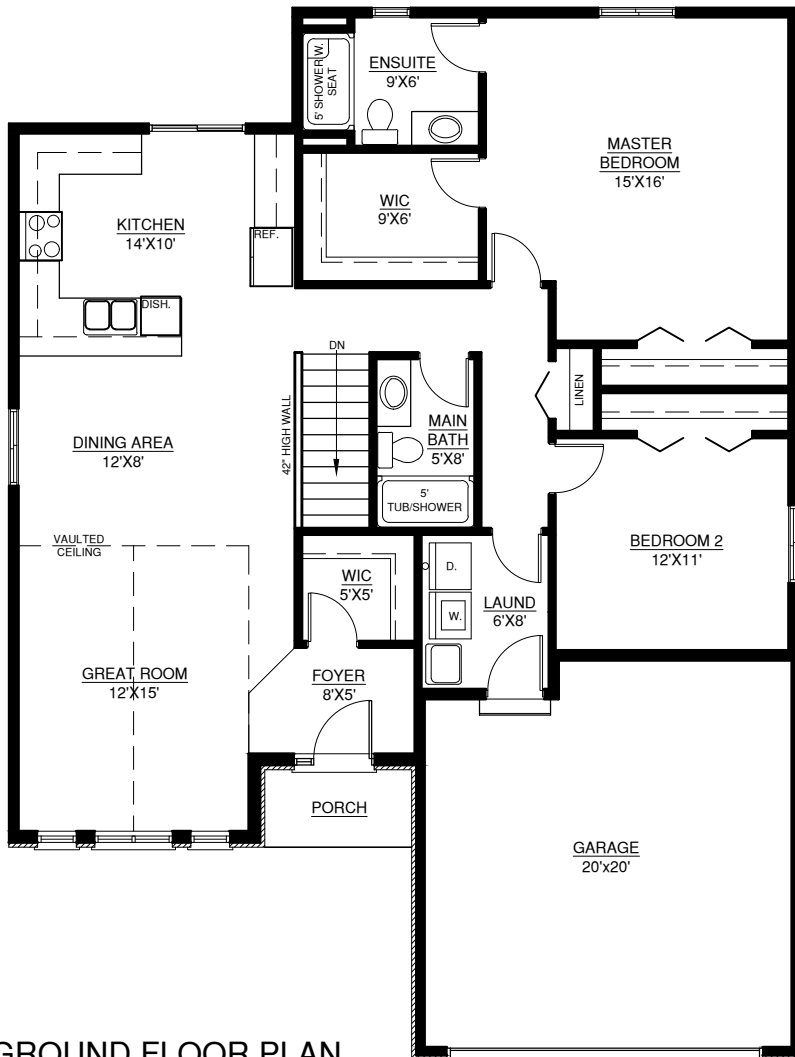
GROUND FLOOR PLAN 40'-10"X54'-5"
