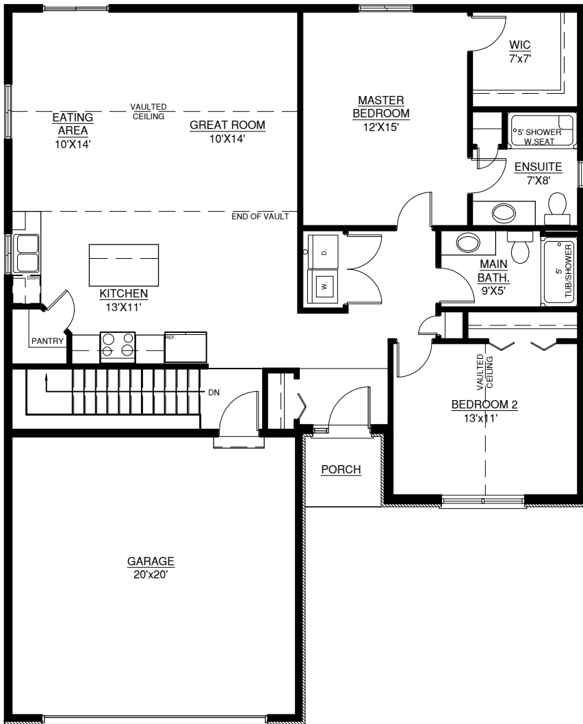
GROUND FLOOR PLAN 42'-0"X52'-0"
