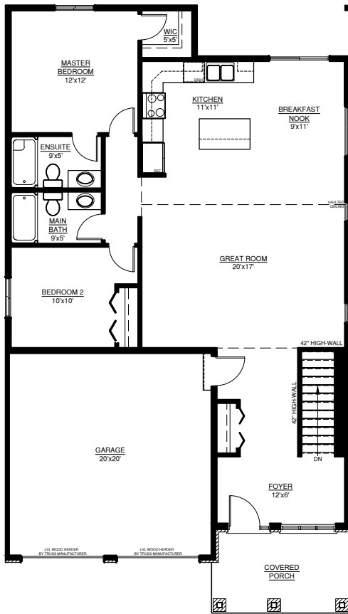
GROUND FLOOR PLAN 34'-0"X60'-0"
