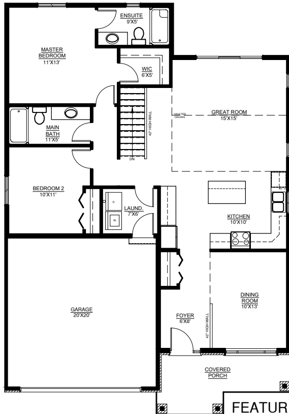
GROUND FLOOR PLAN 38'-4"X55'-1"
