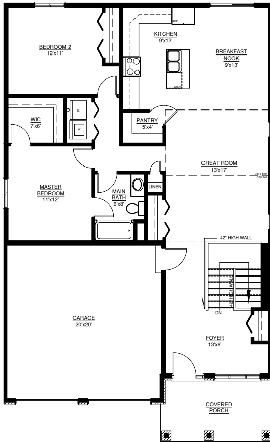
GROUND FLOOR PLAN 35'-0"X57'-0"
