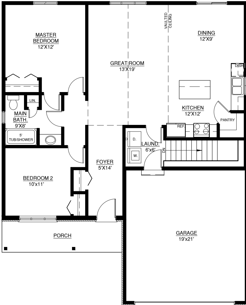
GROUND FLOOR PLAN 39'-7"X49'-0"
