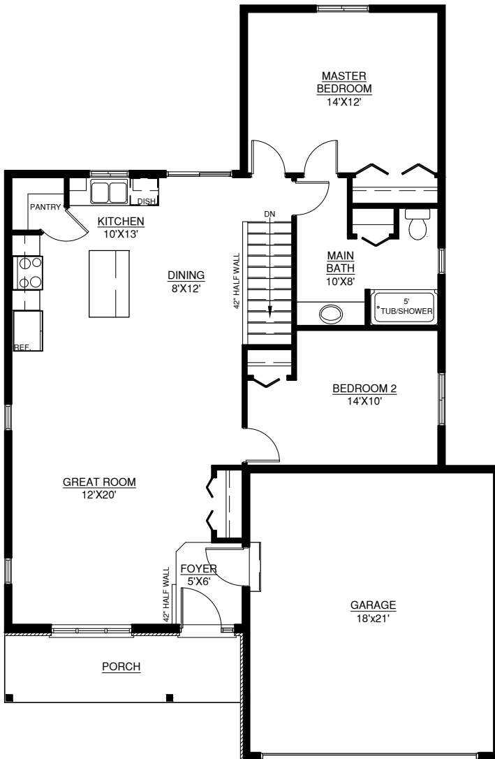
GROUND FLOOR PLAN 37'-0"X56'-8"
